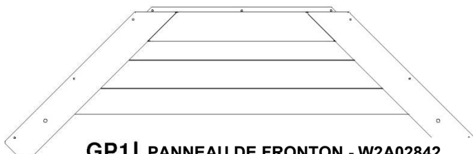
GP1 | PANNEAU DE FRONTON - W2A02842 (x2) | 1 1/8" x 16 3/8" x 53 1/2" (27x414x1359)
